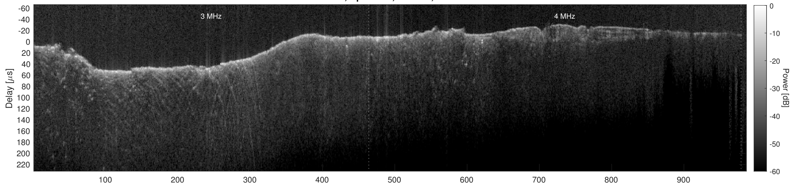
Orbit 4670, Cluttergram
