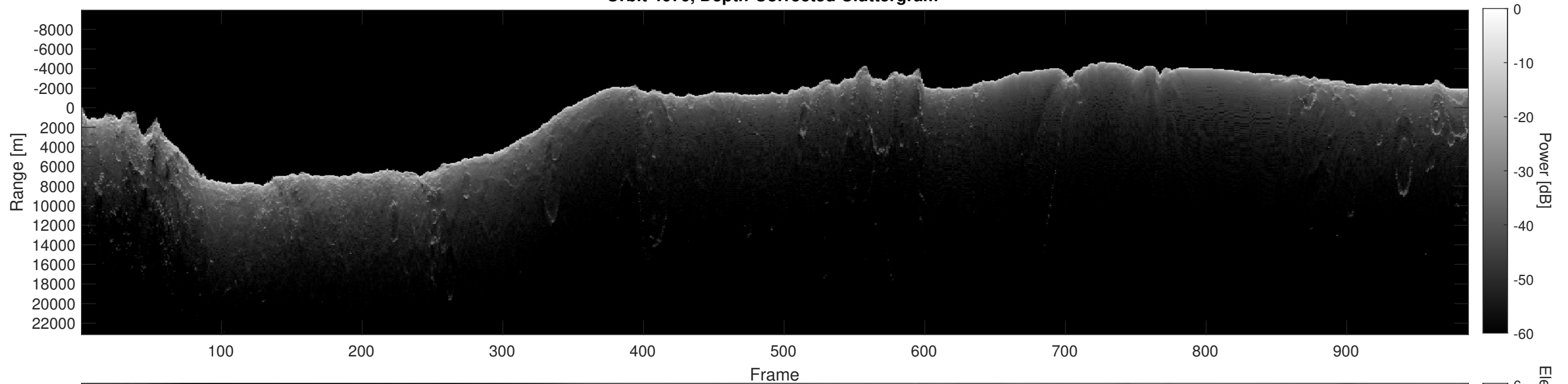
Orbit 4670, Depth-Corrected Cluttergram
