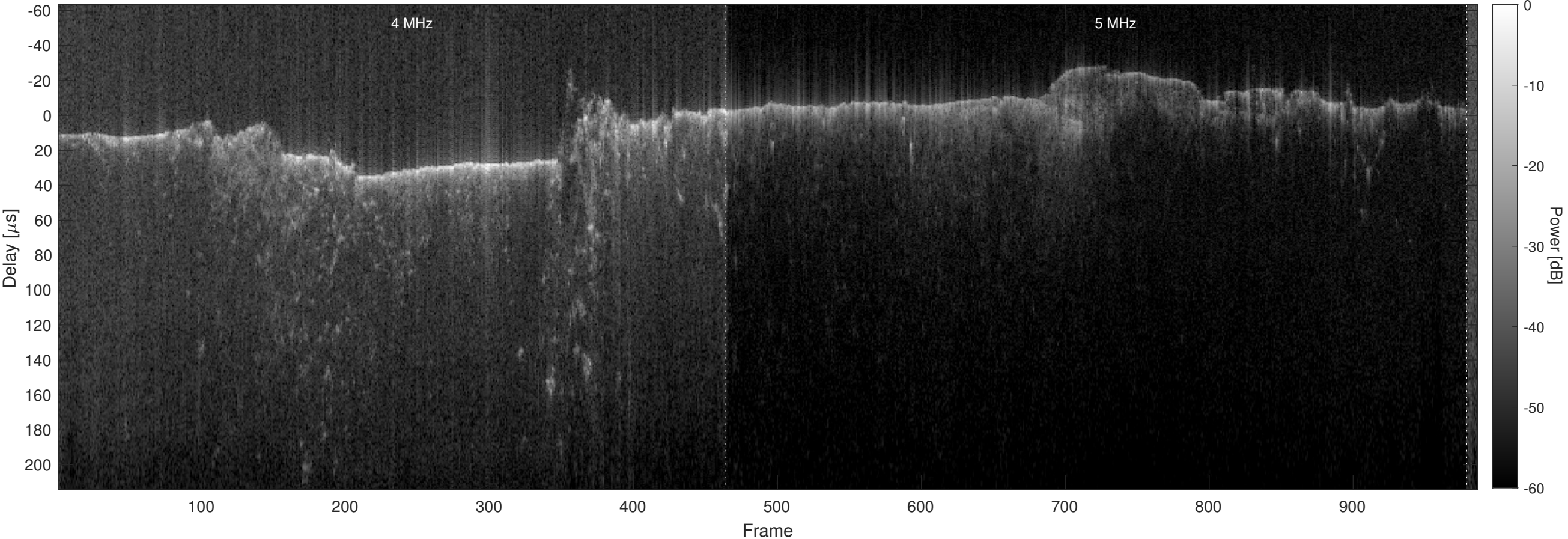
Orbit 4671, Optimized, No Window, Channel 2
