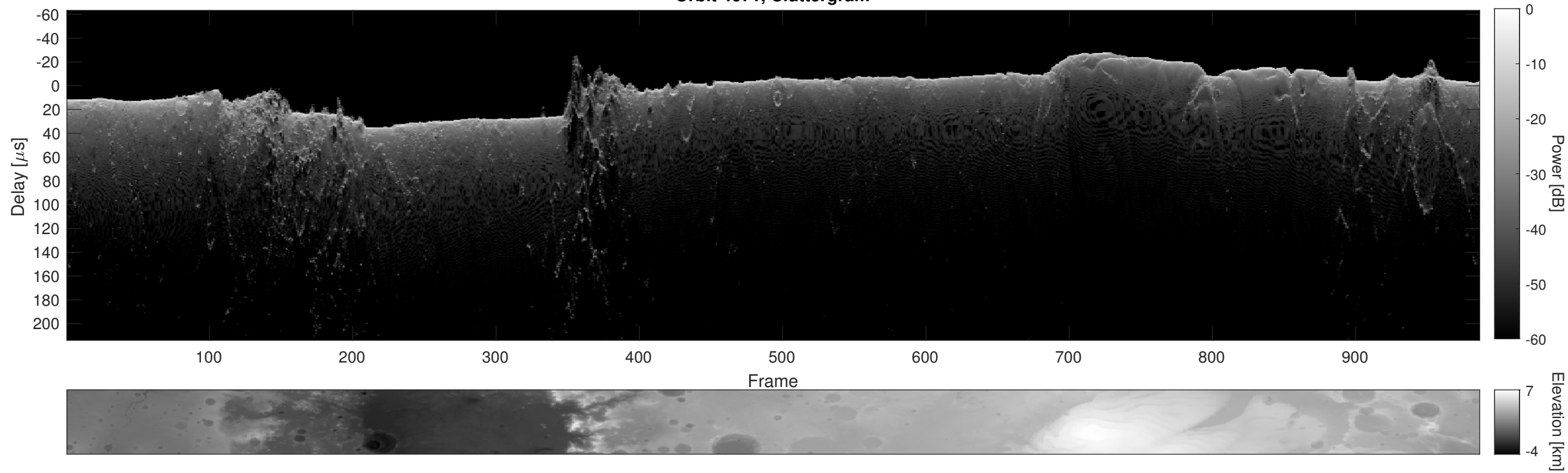
Orbit 4671, Cluttergram
