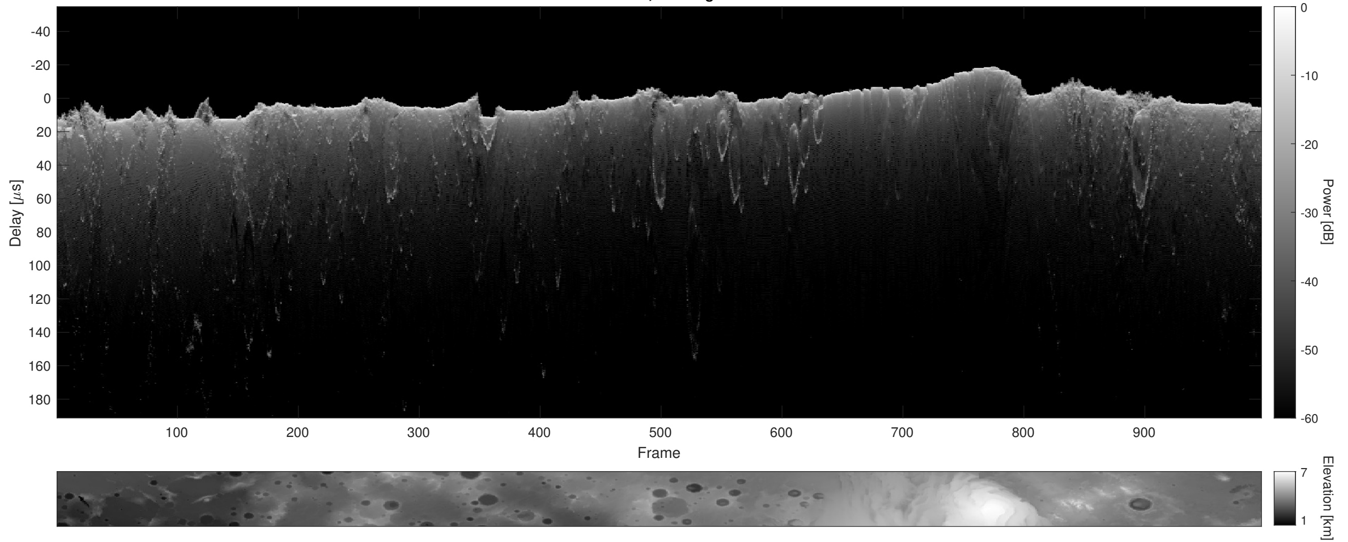
Orbit 4672, Cluttergram
