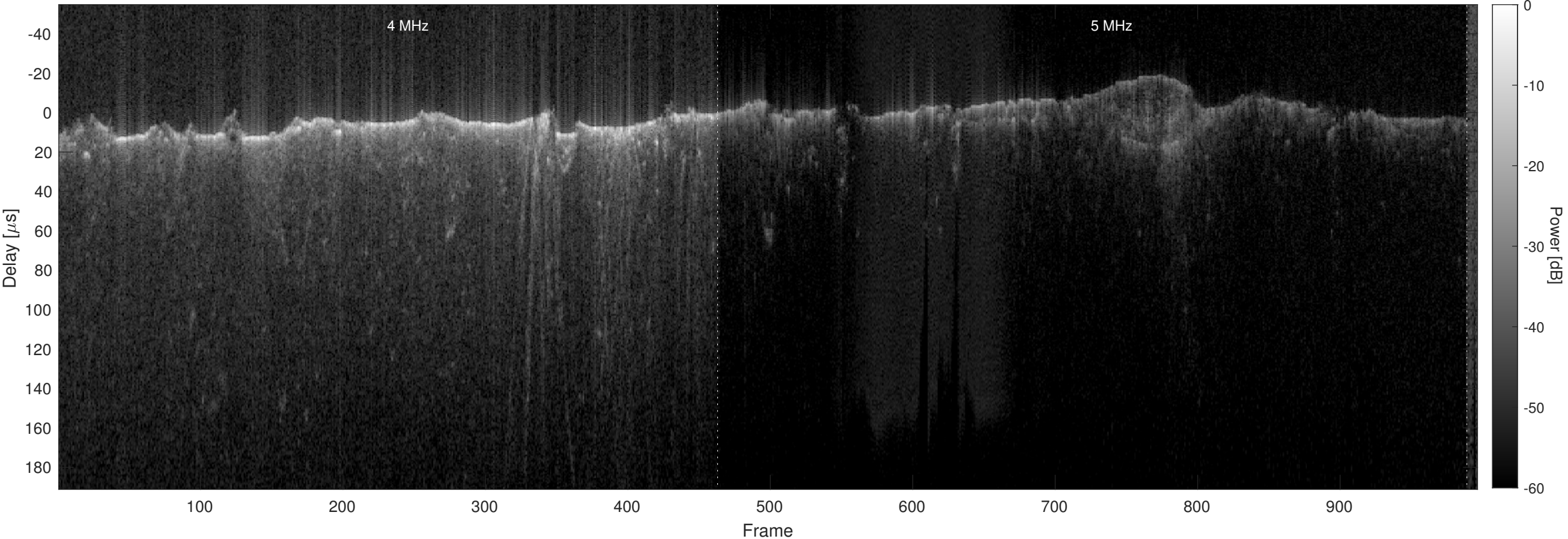
Orbit 4672, Optimized, No Window, Channel 2
