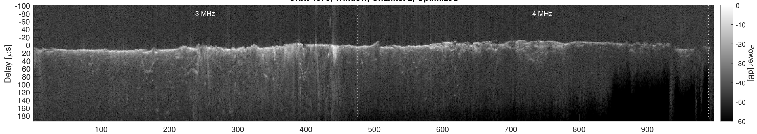
Orbit 4673, Cluttergram
