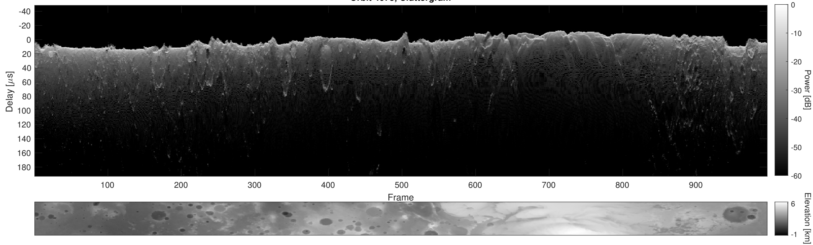
Orbit 4673, Cluttergram
