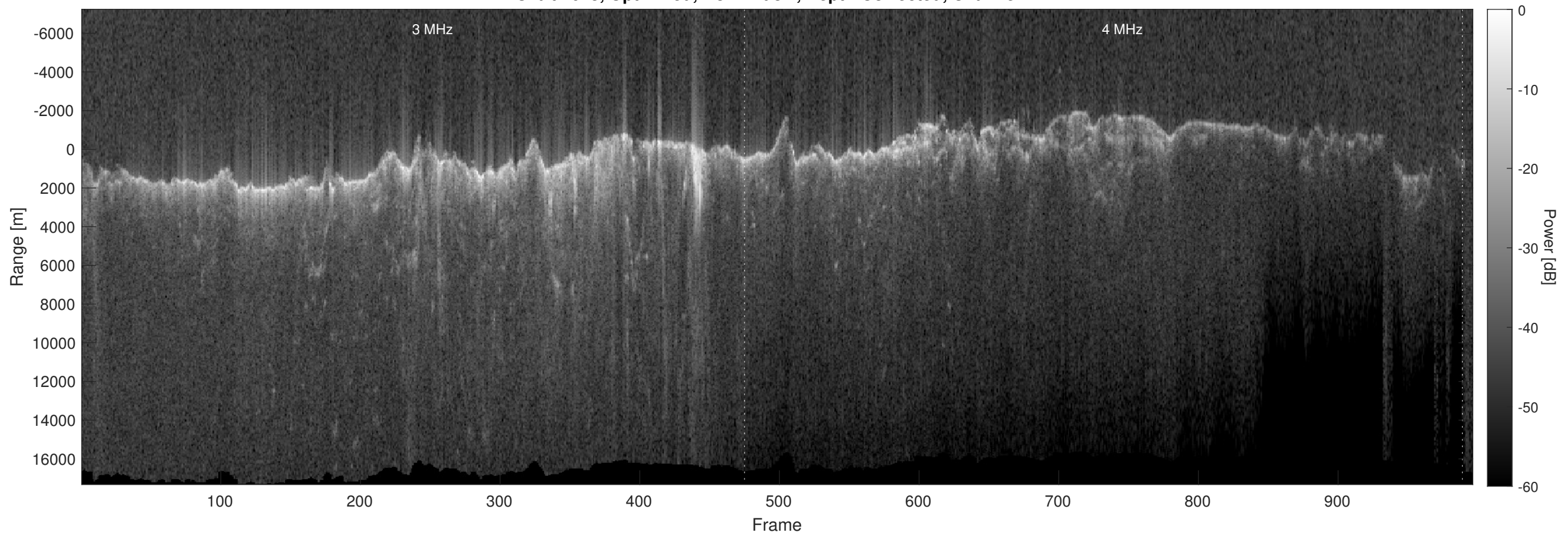
Orbit 4673, Optimized, No Window, Depth-Corrected, Channel 2
