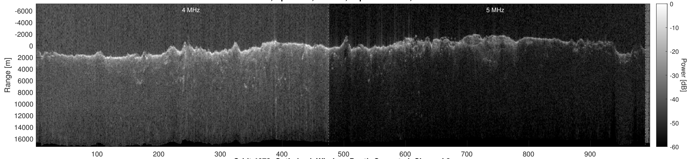
Orbit 4673, Optimized, Window, Depth-Corrected, Channel 2
