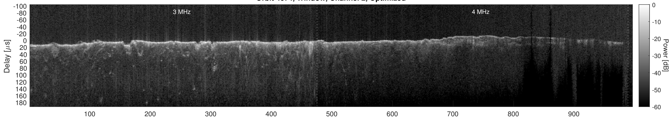
Orbit 4674, Cluttergram
