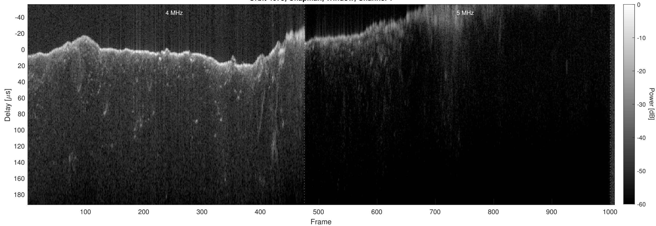
Orbit 4675, Chapman, Window, Channel 2
