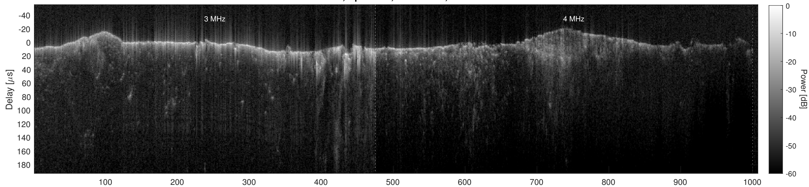
Orbit 4675, Cluttergram
