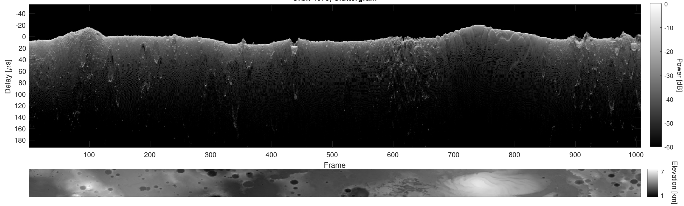
Orbit 4675, Cluttergram
