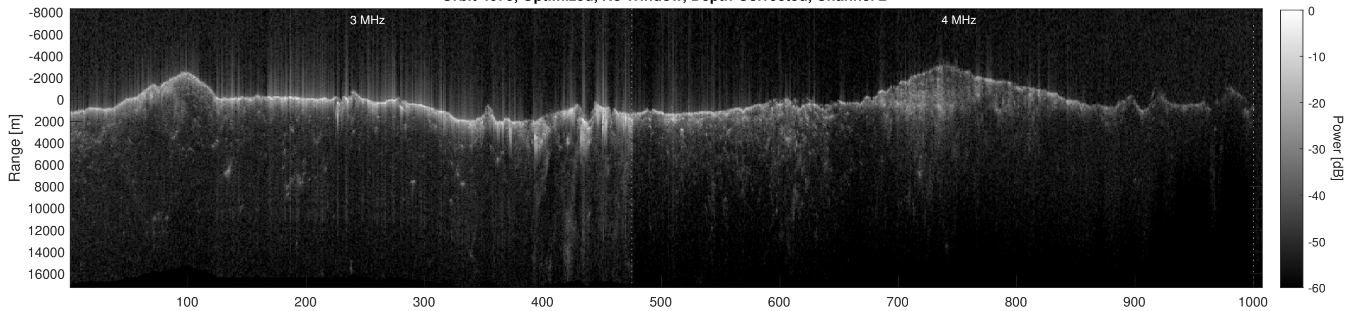
Orbit 4675, Depth-Corrected Cluttergram
