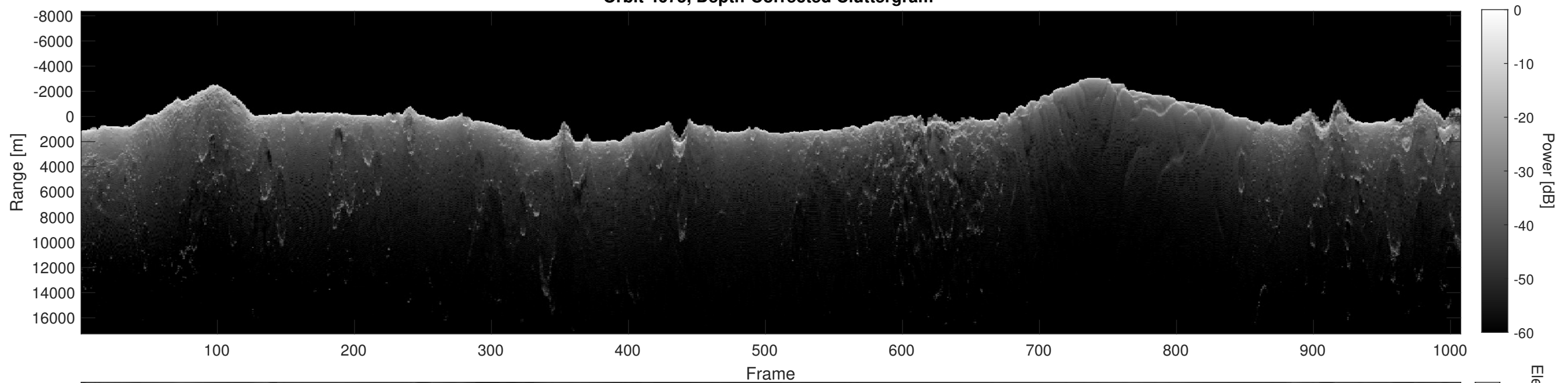
Orbit 4675, Depth-Corrected Cluttergram
