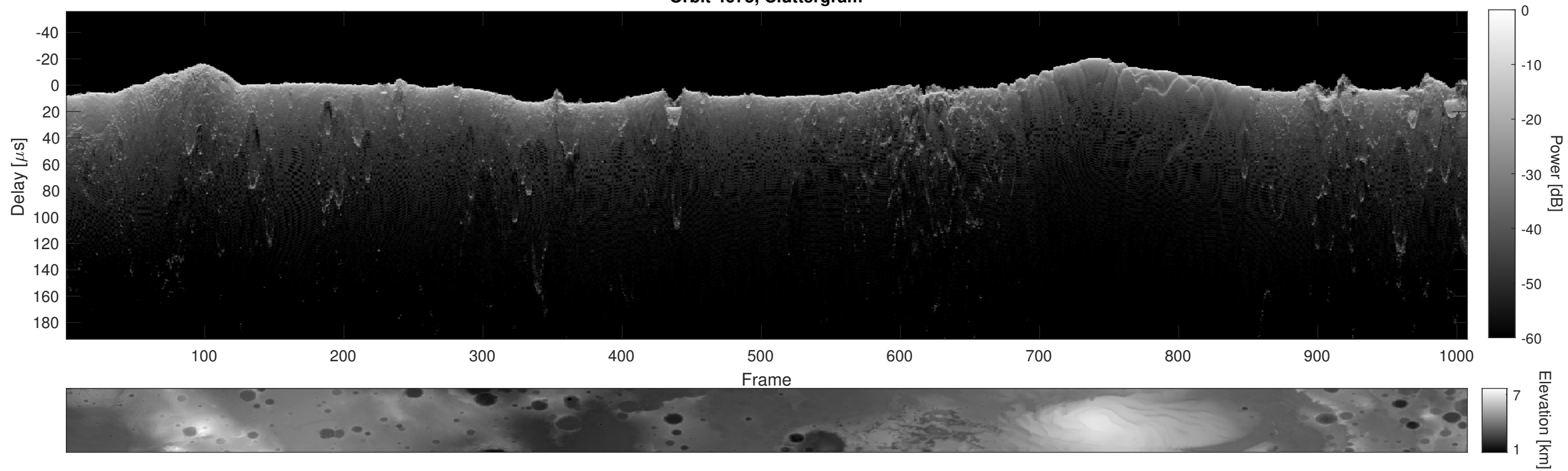
Orbit 4675, Cluttergram
