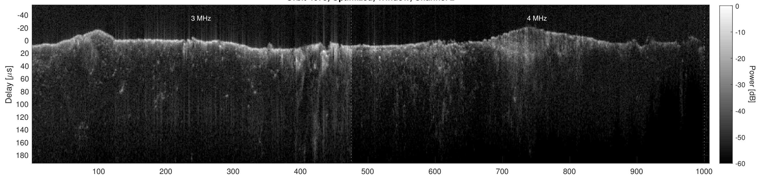
Orbit 4675, Cluttergram
