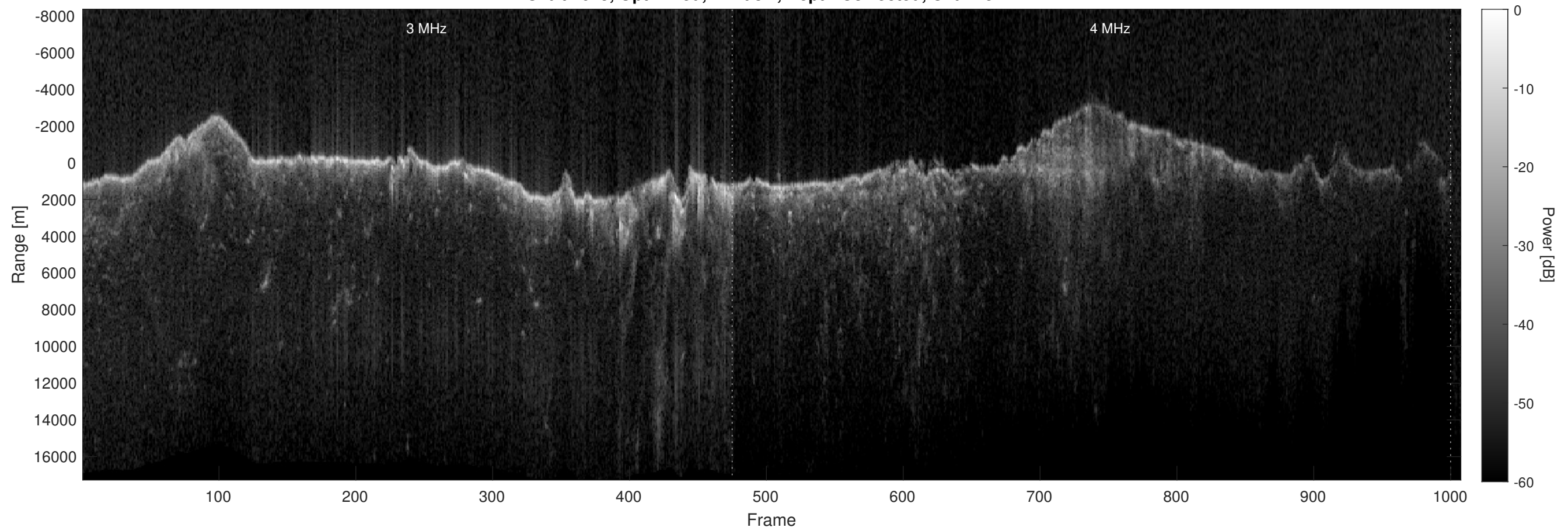
Orbit 4675, Optimized, Window, Depth-Corrected, Channel 2
