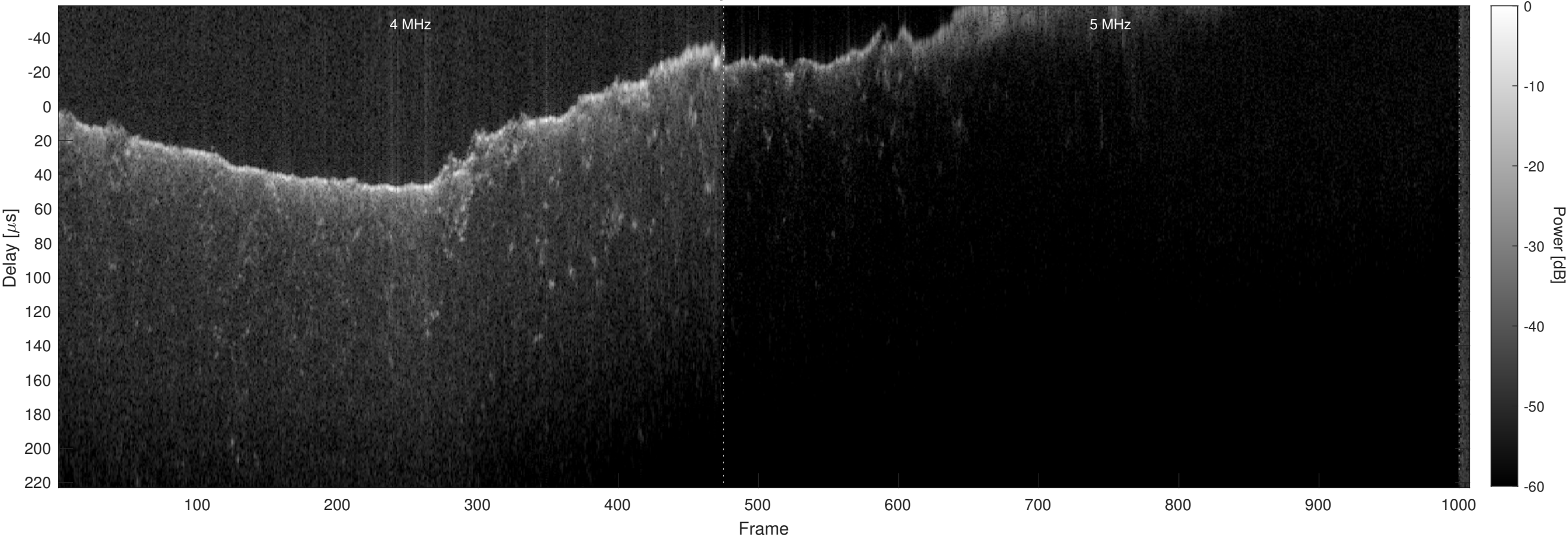
Orbit 4677, Chapman, Window, Channel 2
