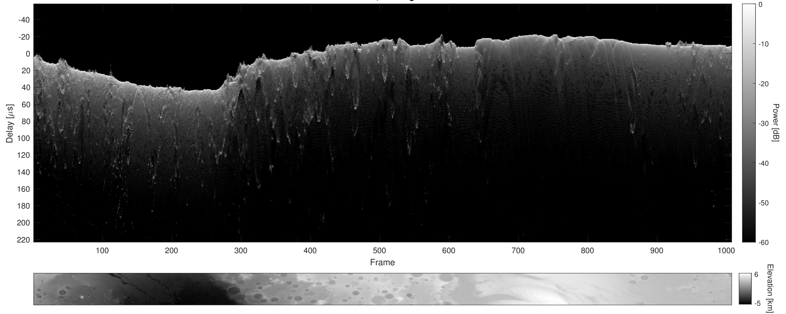
Orbit 4677, Cluttergram
