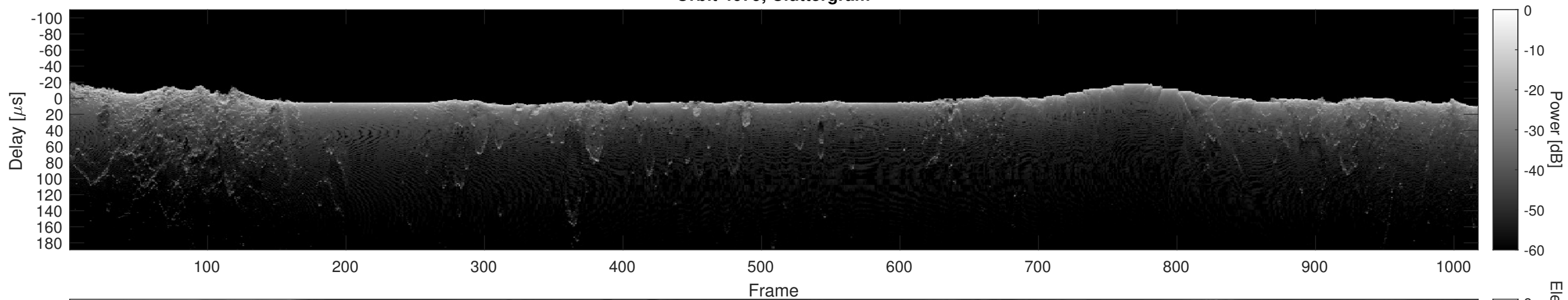
Orbit 4679, Cluttergram
