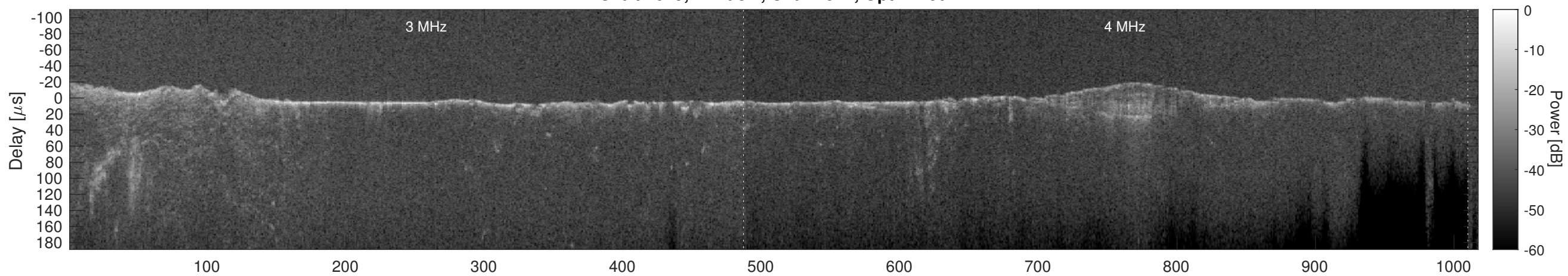
Orbit 4679, Cluttergram
