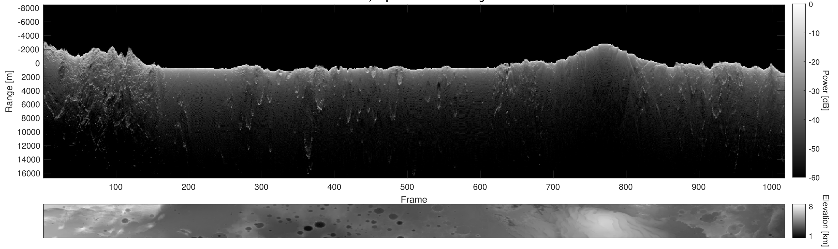
Orbit 4679, Depth-Corrected Cluttergram
