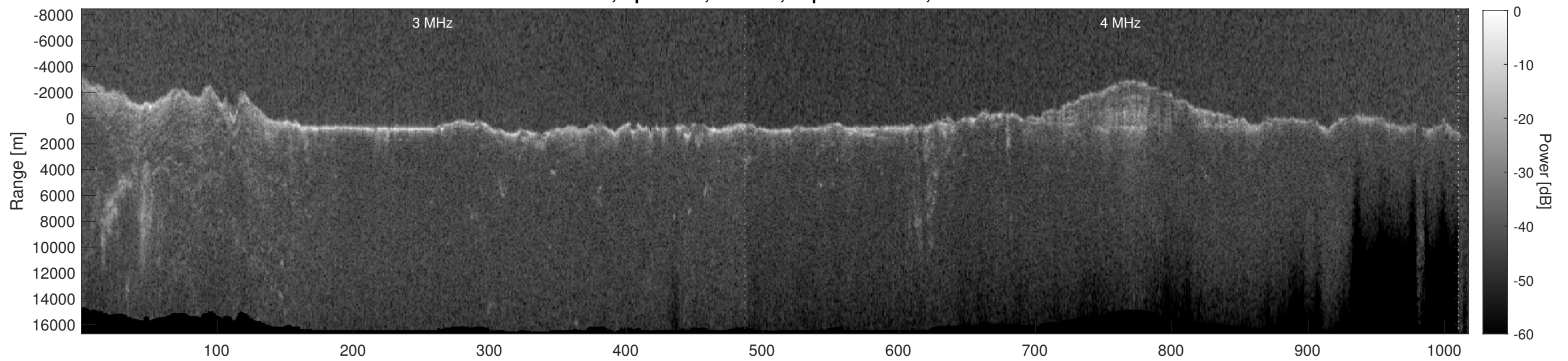
Orbit 4679, Depth-Corrected Cluttergram
