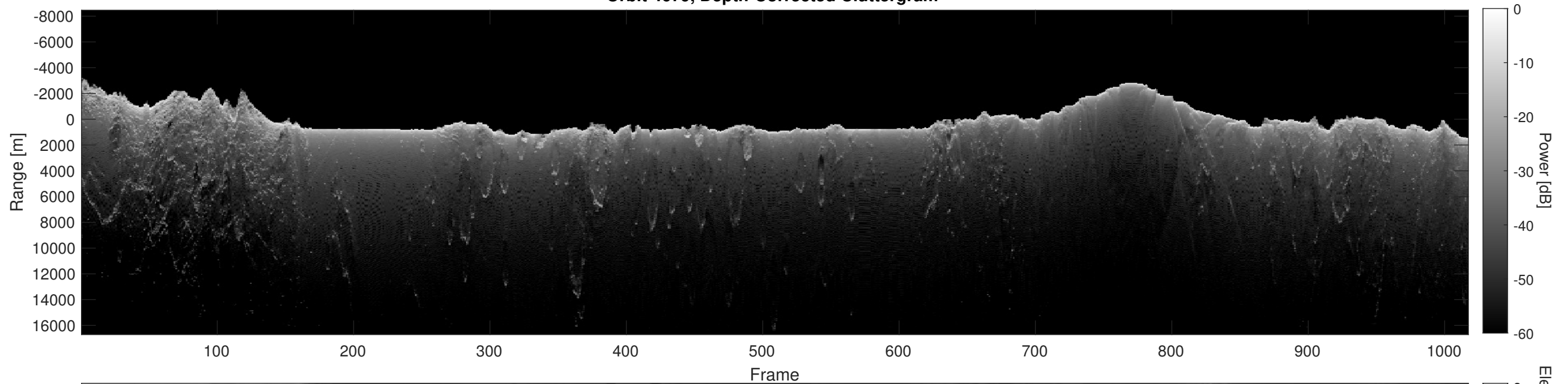
Orbit 4679, Depth-Corrected Cluttergram
