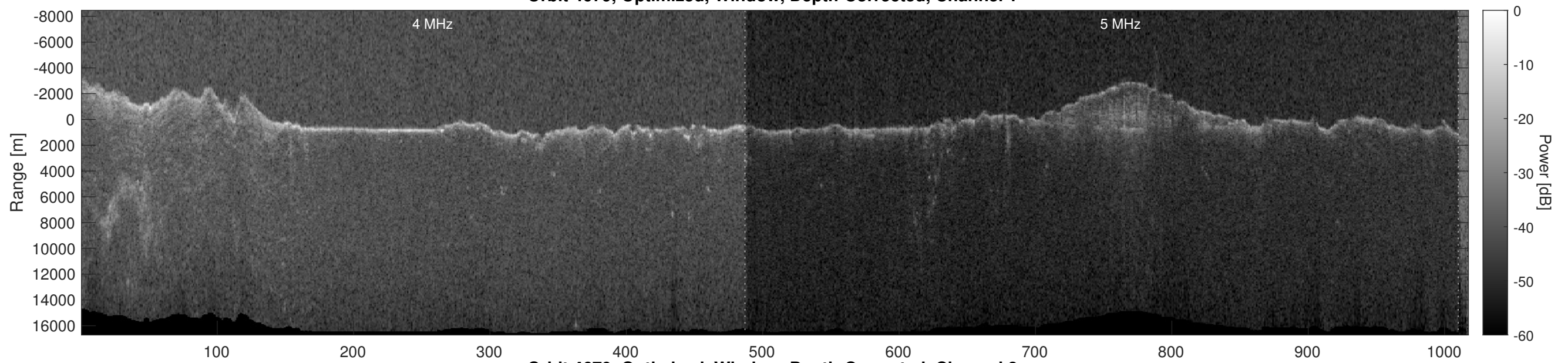
Orbit 4679, Optimized, Window, Depth-Corrected, Channel 2
