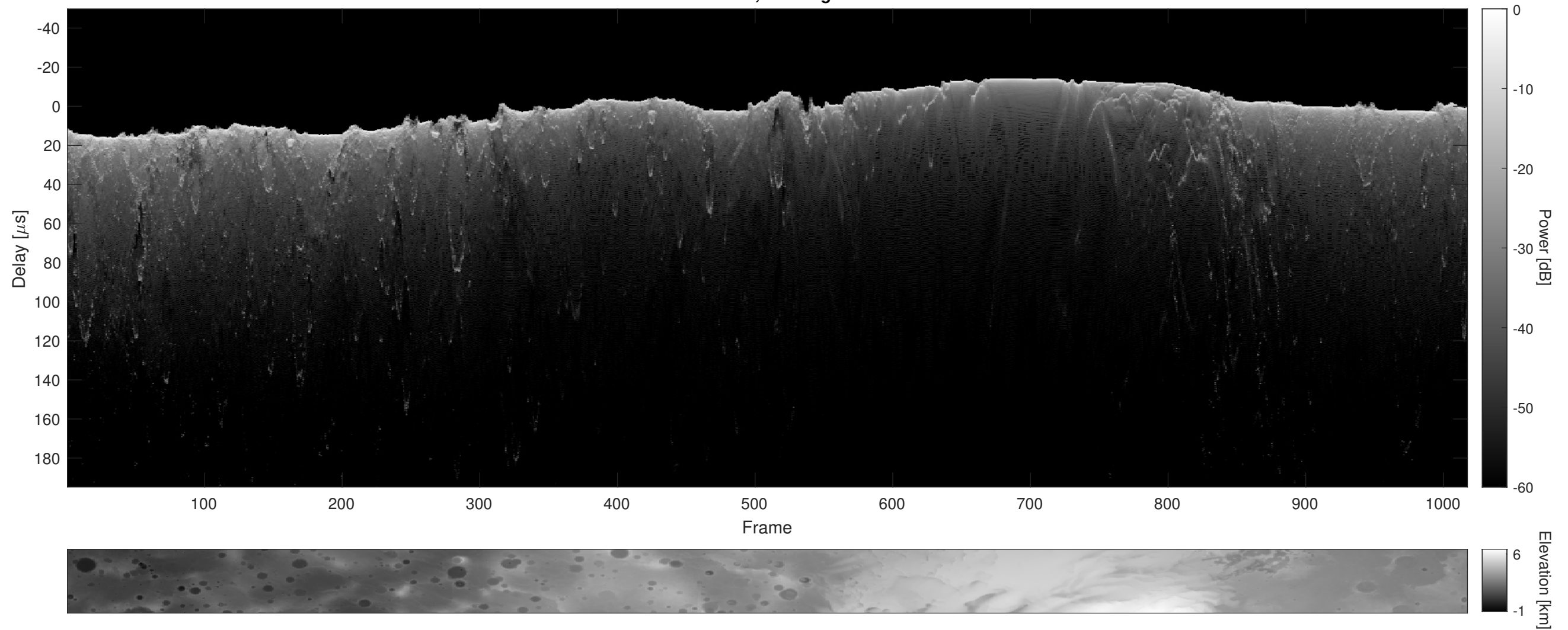
Orbit 4680, Cluttergram
