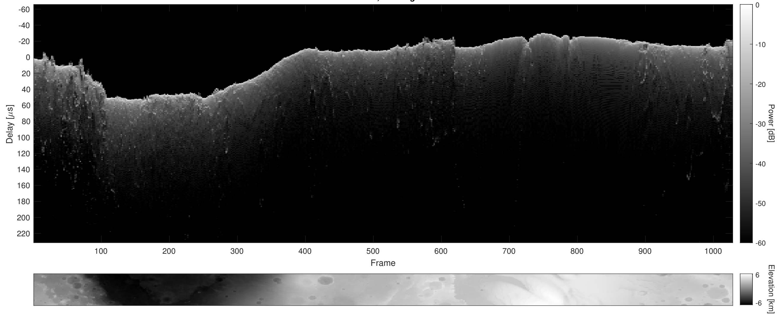
Orbit 4681, Cluttergram
