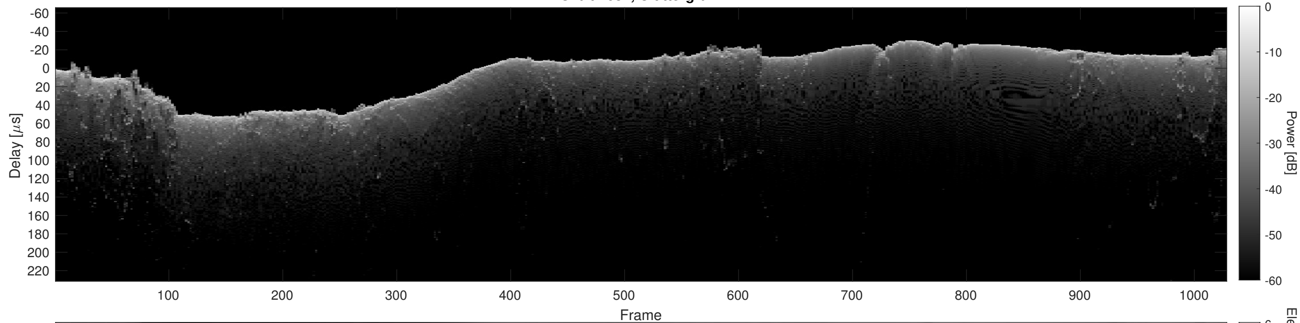
Orbit 4681, Cluttergram
