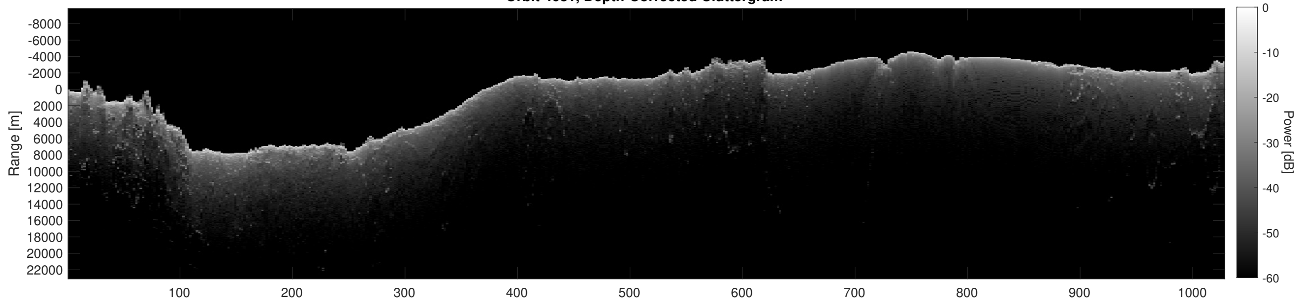
Orbit 4681, Depth-Corrected Cluttergram
