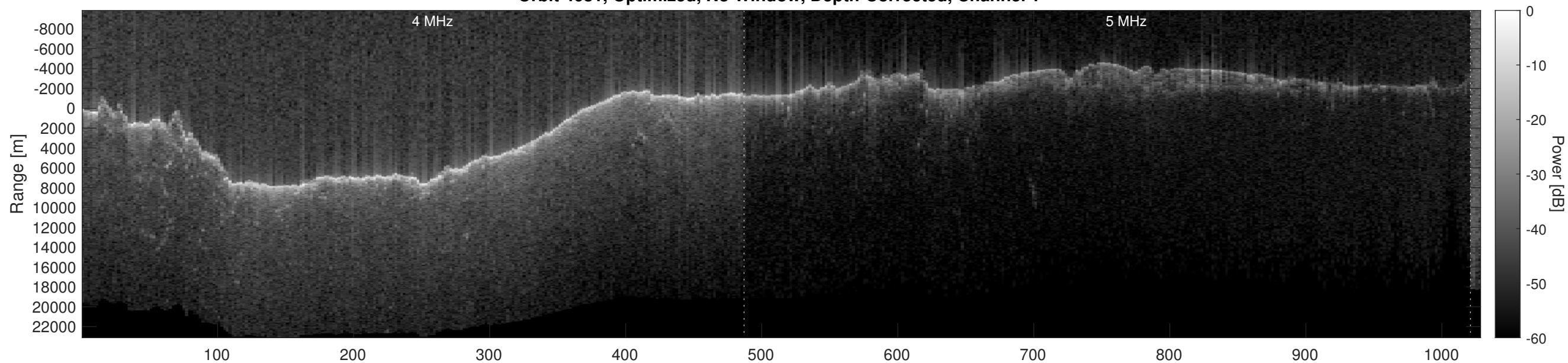
Orbit 4681, Optimized, No Window, Depth-Corrected, Channel 2
