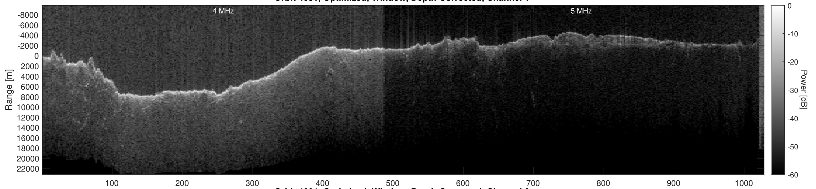
Orbit 4681, Optimized, Window, Depth-Corrected, Channel 2
