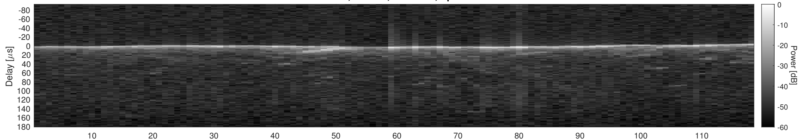
Orbit 4682, Cluttergram
