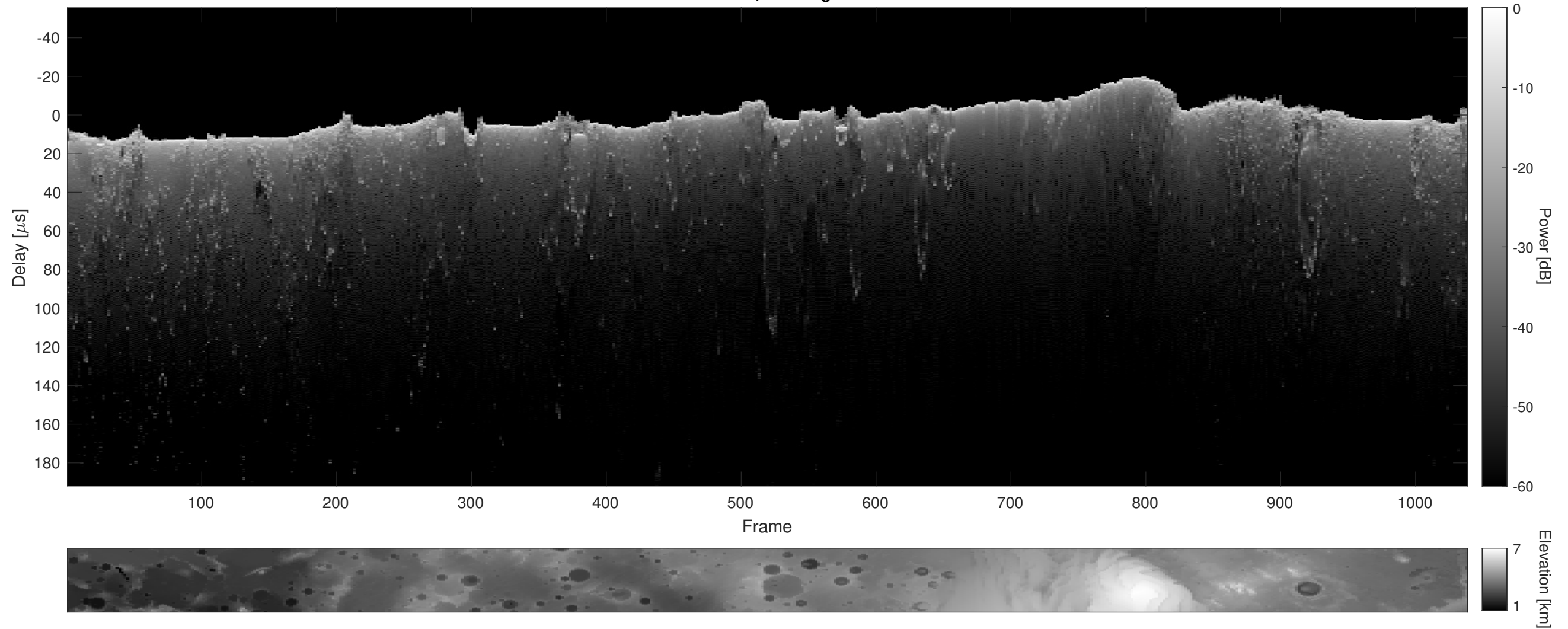
Orbit 4683, Cluttergram
