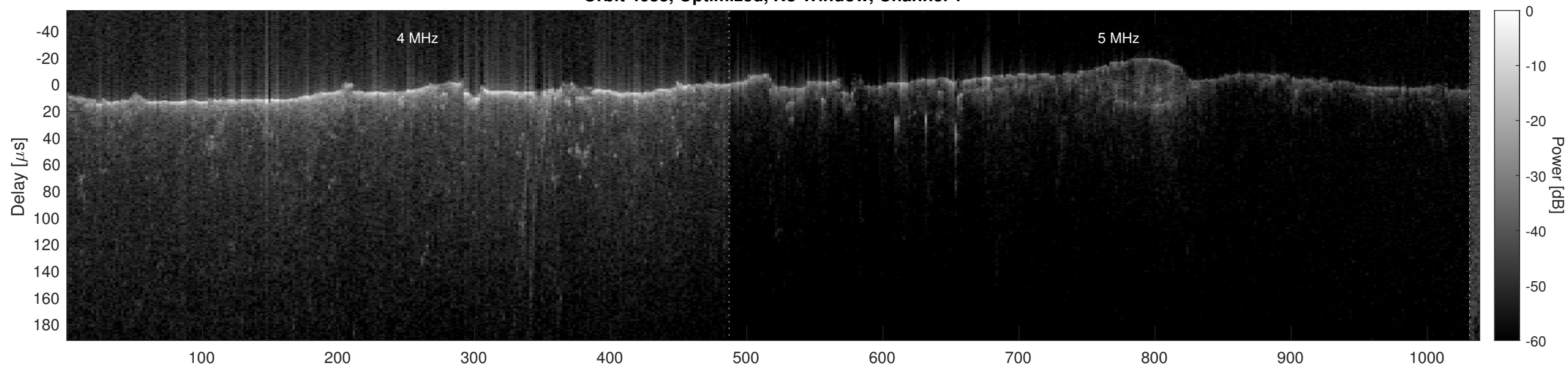
Orbit 4683, Optimized, No Window, Channel 2
