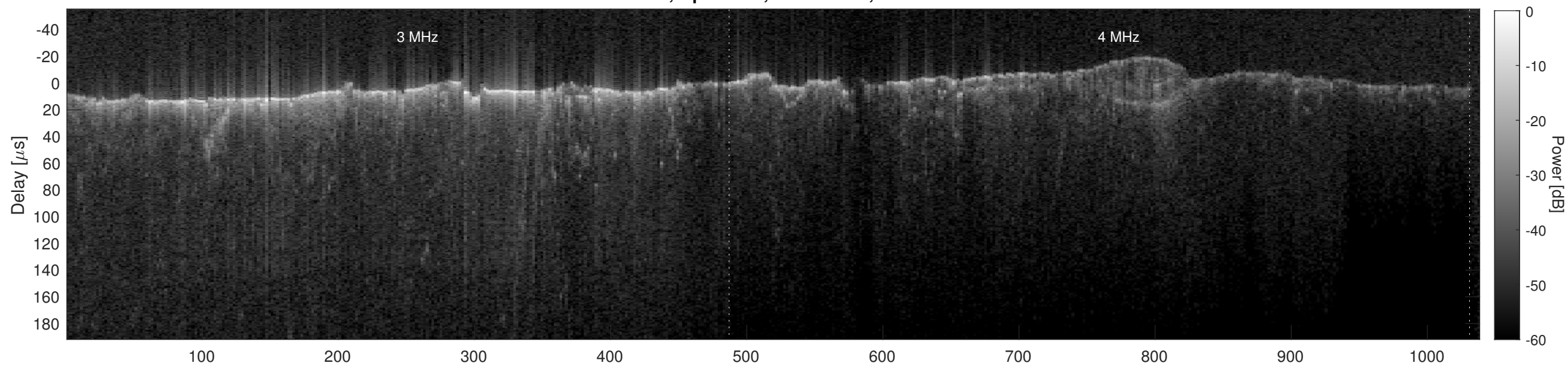
Orbit 4683, Cluttergram
