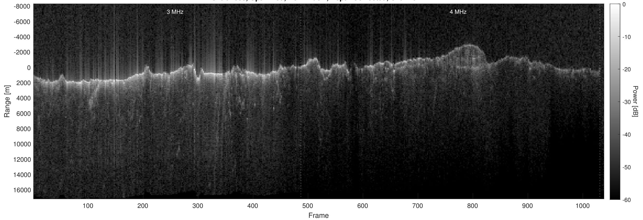
Orbit 4683, Optimized, No Window, Depth-Corrected, Channel 2
