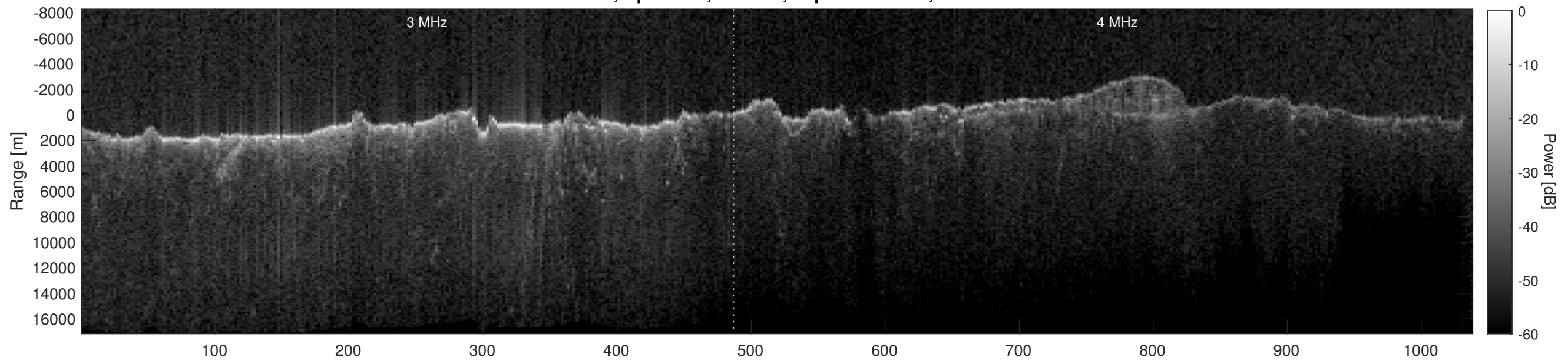
Orbit 4683, Depth-Corrected Cluttergram
