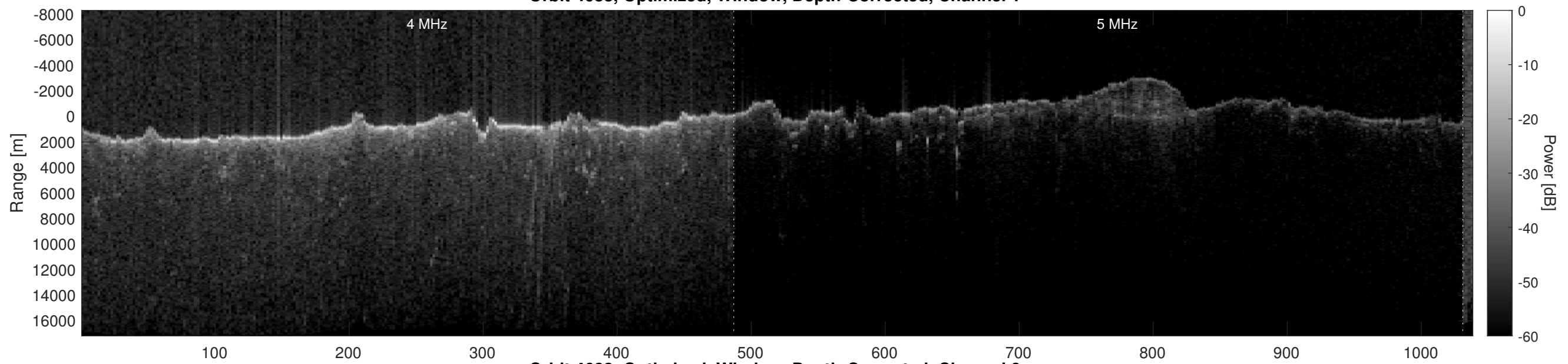
Orbit 4683, Optimized, Window, Depth-Corrected, Channel 2
