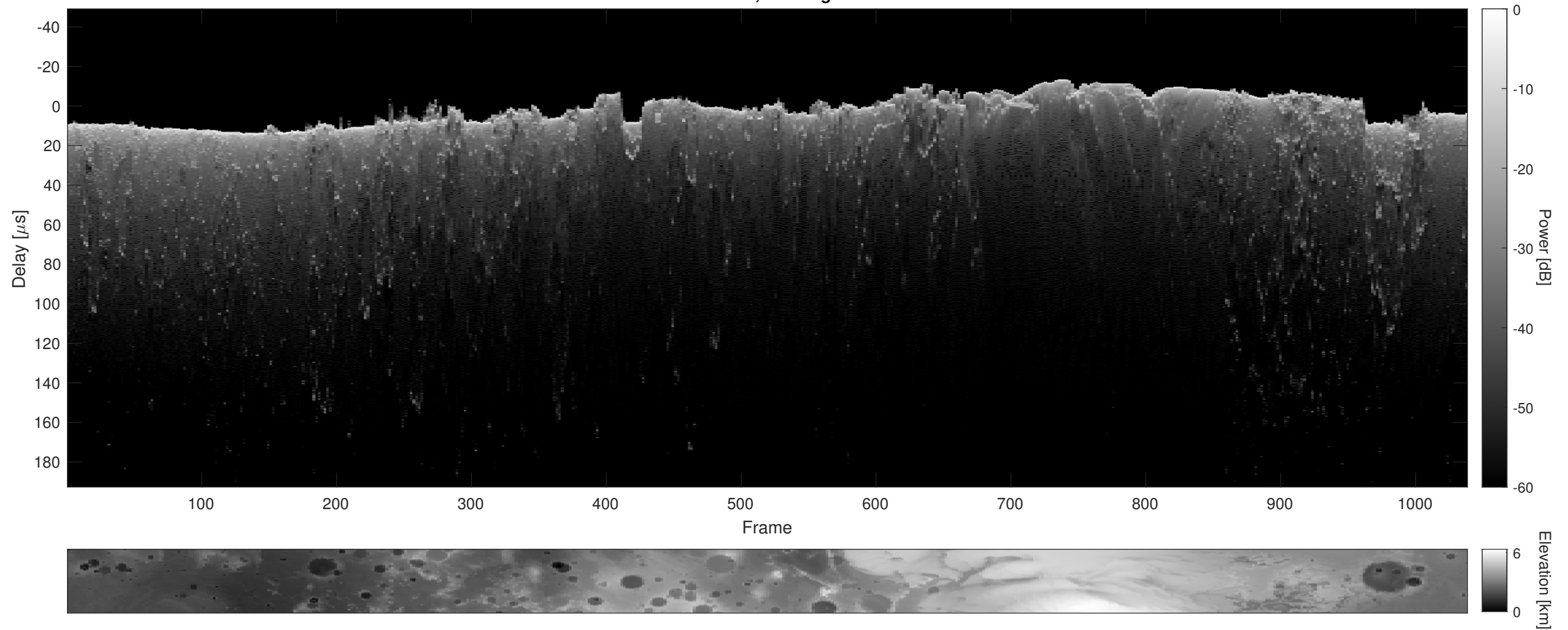
Orbit 4684, Cluttergram
