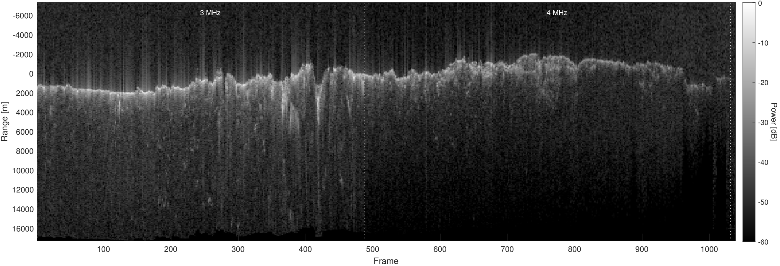
Orbit 4684, Optimized, No Window, Depth-Corrected, Channel 2
