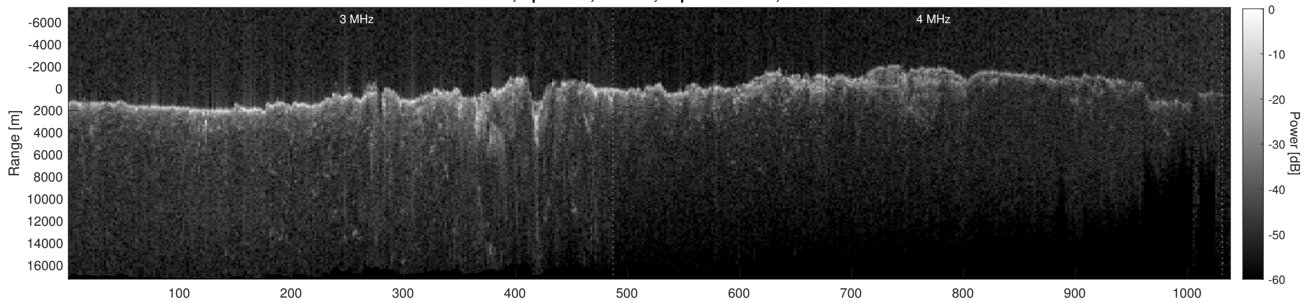
Orbit 4684, Depth-Corrected Cluttergram
