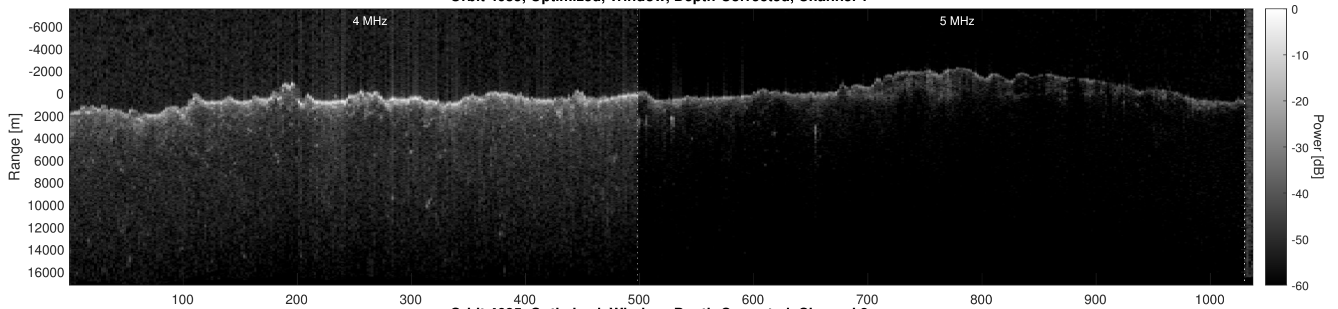
Orbit 4685, Optimized, Window, Depth-Corrected, Channel 2
