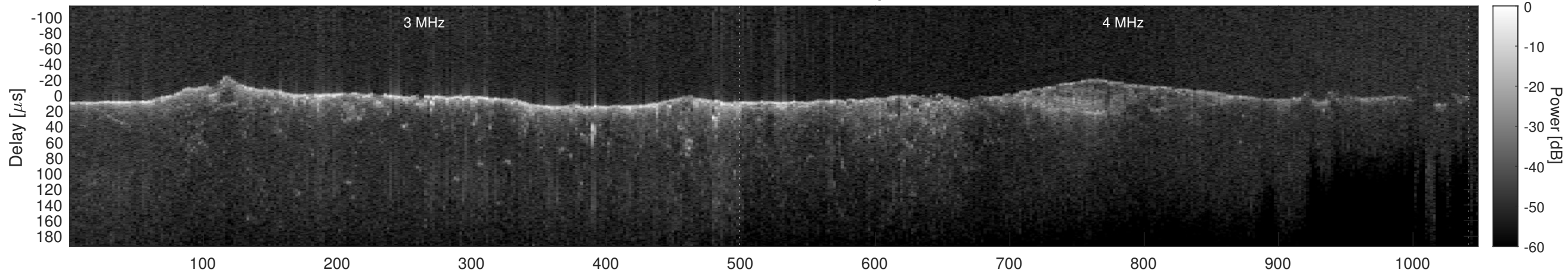
Orbit 4686, Cluttergram
