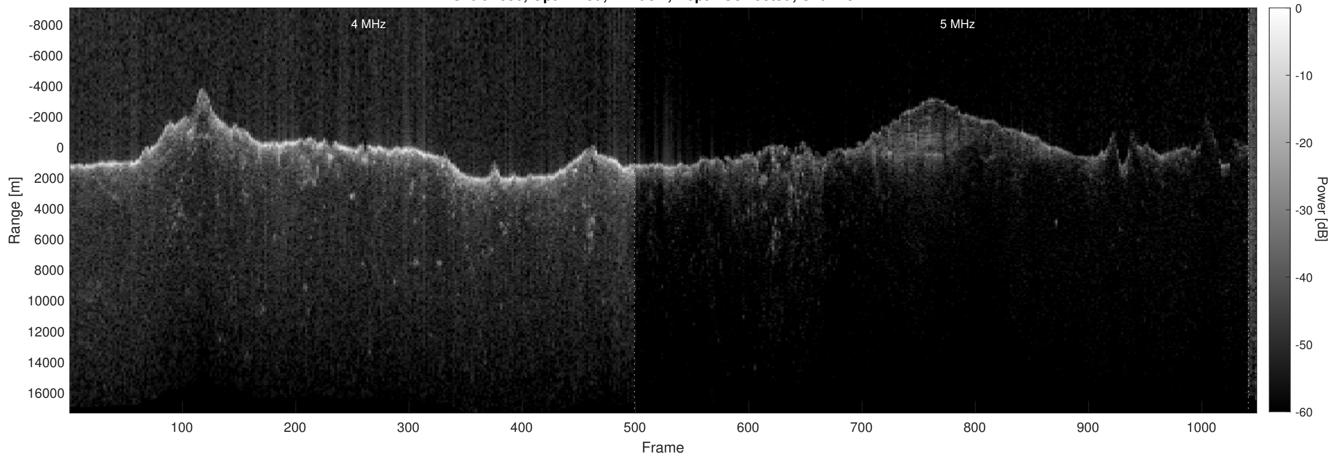
Orbit 4686, Optimized, Window, Depth-Corrected, Channel 2
