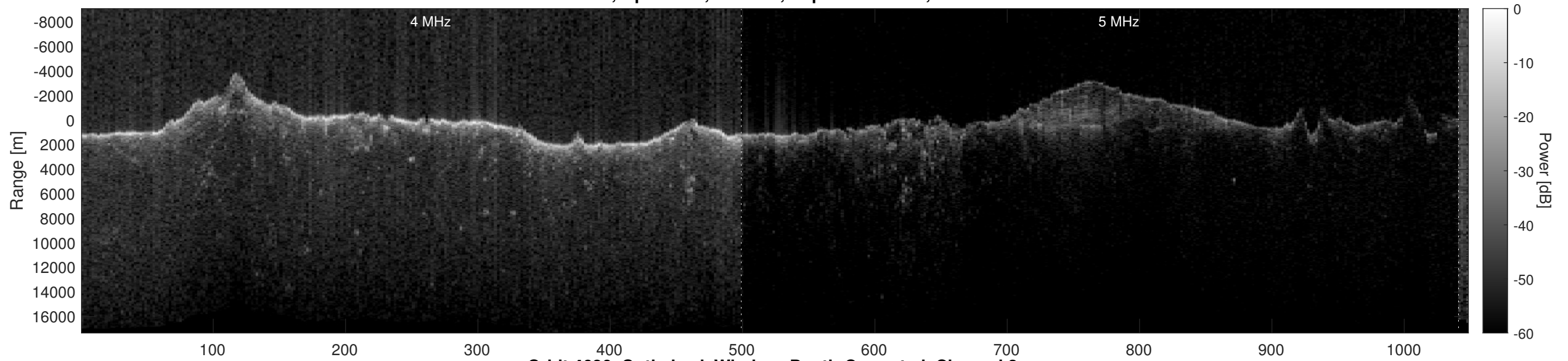
Orbit 4686, Optimized, Window, Depth-Corrected, Channel 2
