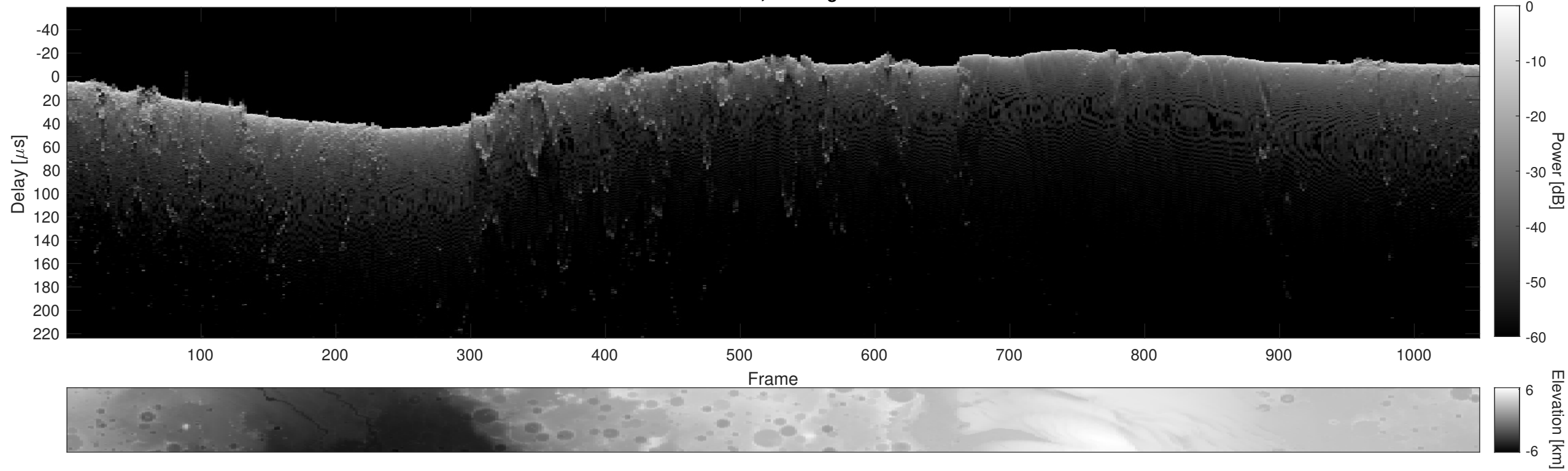
Orbit 4688, Cluttergram
