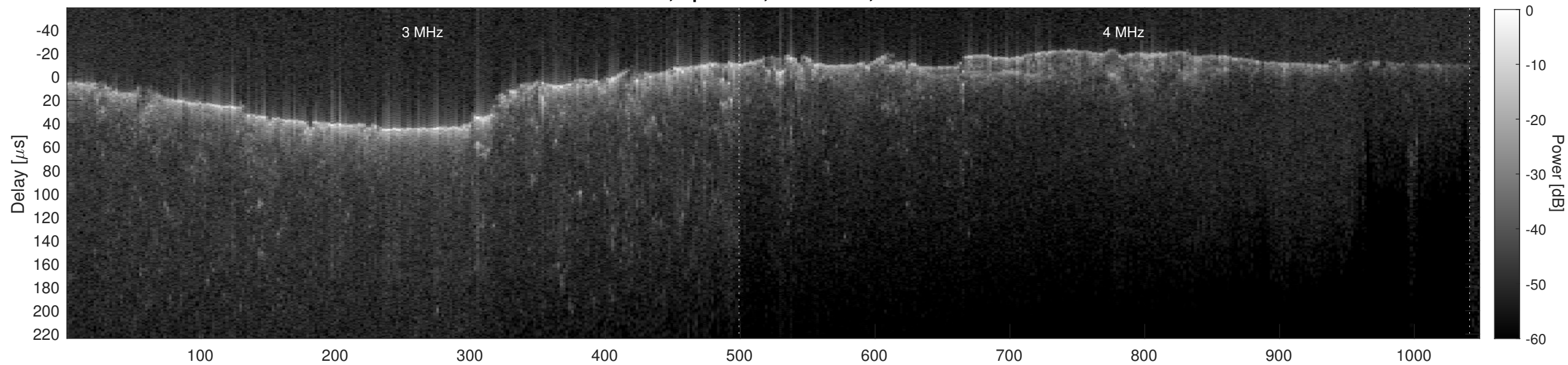
Orbit 4688, Cluttergram
