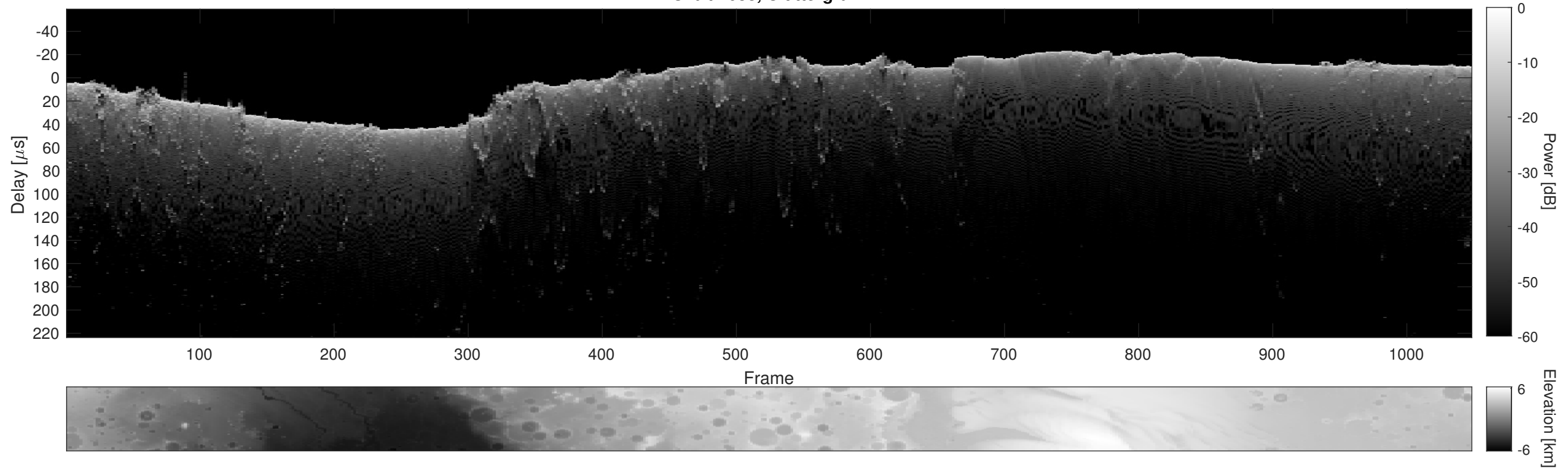
Orbit 4688, Cluttergram
