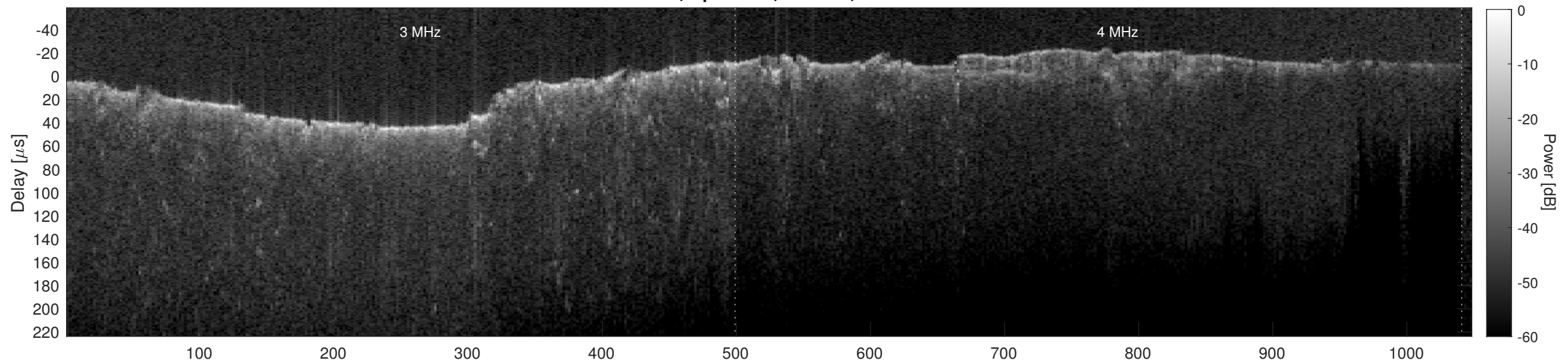
Orbit 4688, Cluttergram
