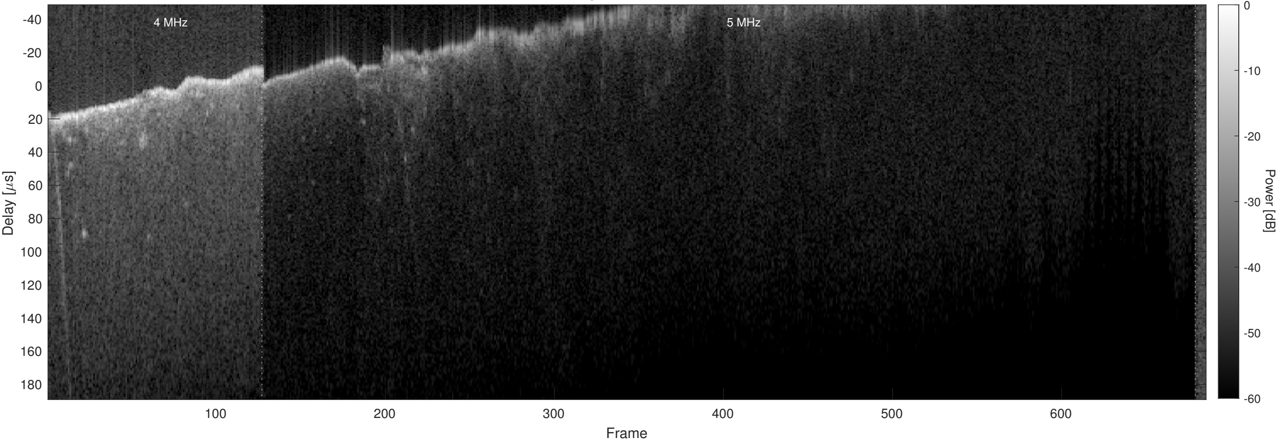
Orbit 4689, Chapman, Window, Channel 2
