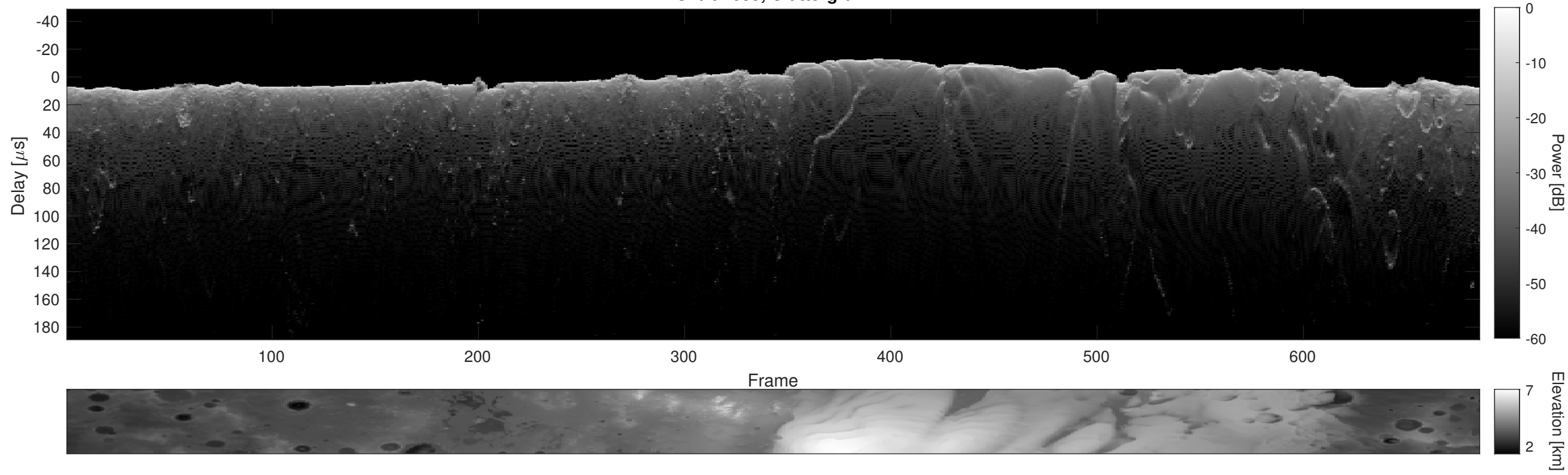
Orbit 4689, Cluttergram
