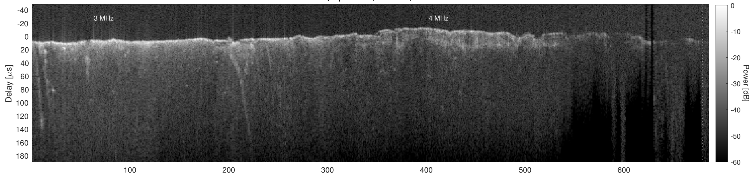
Orbit 4689, Cluttergram
