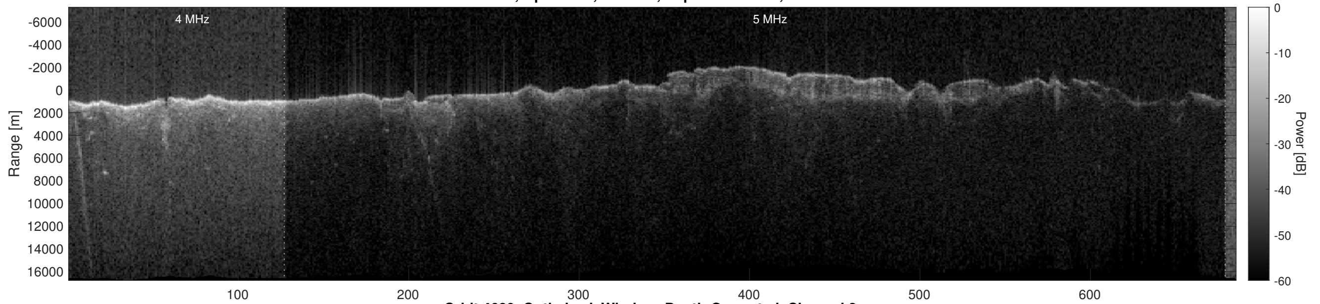
Orbit 4689, Optimized, Window, Depth-Corrected, Channel 2
