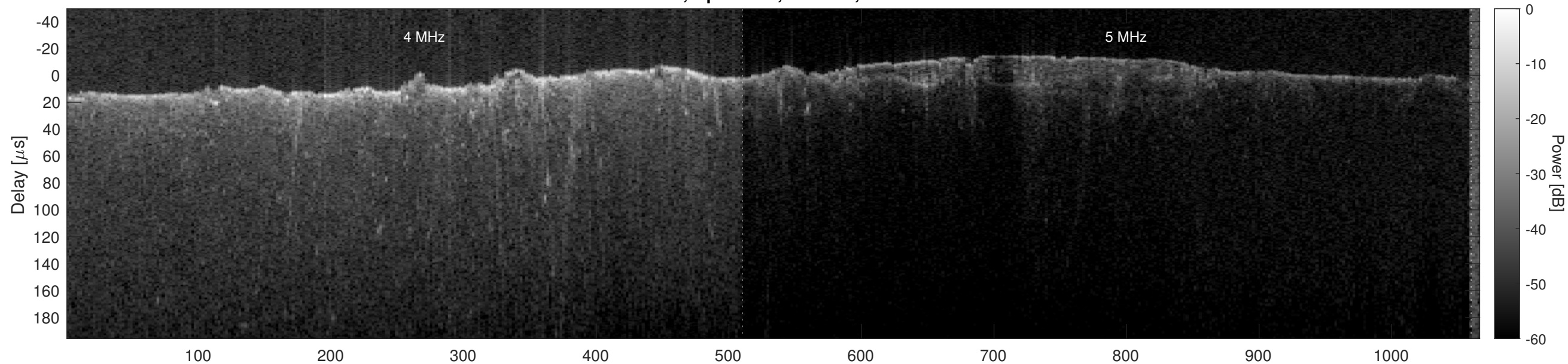
Orbit 4691, Optimized, Window, Channel 2
