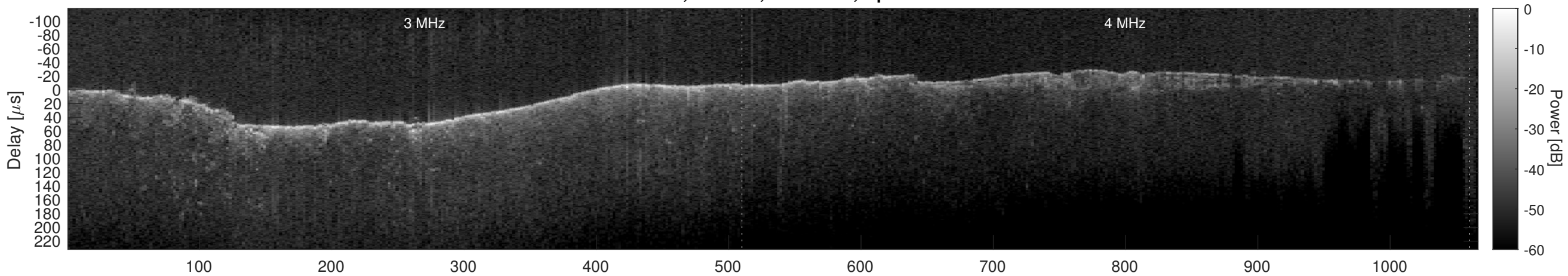
Orbit 4692, Cluttergram
