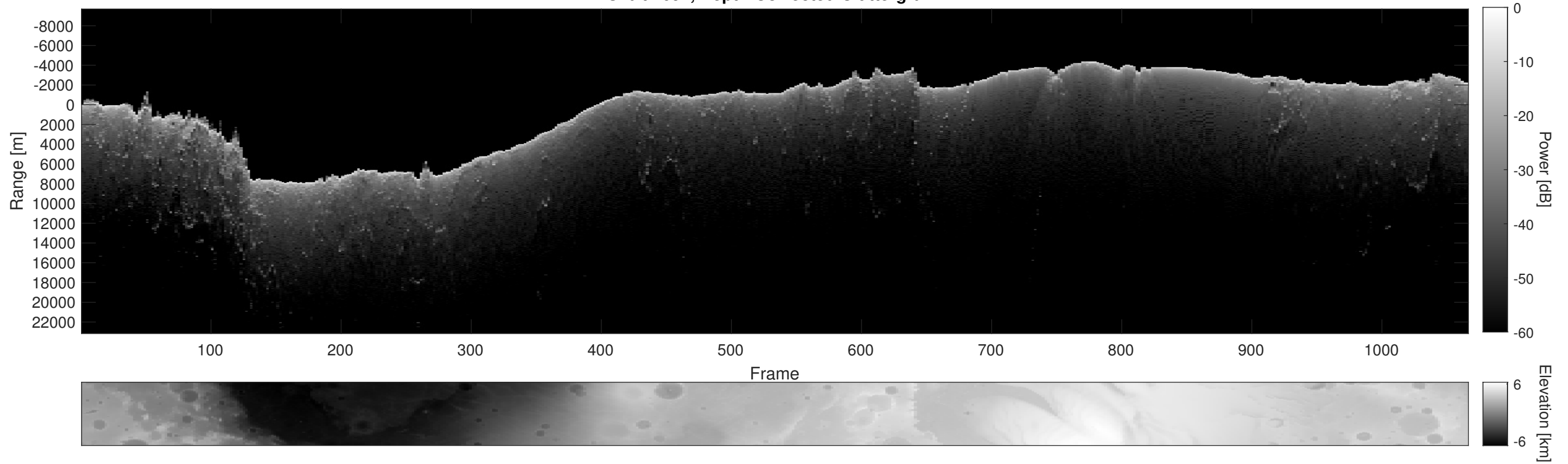
Orbit 4692, Depth-Corrected Cluttergram
