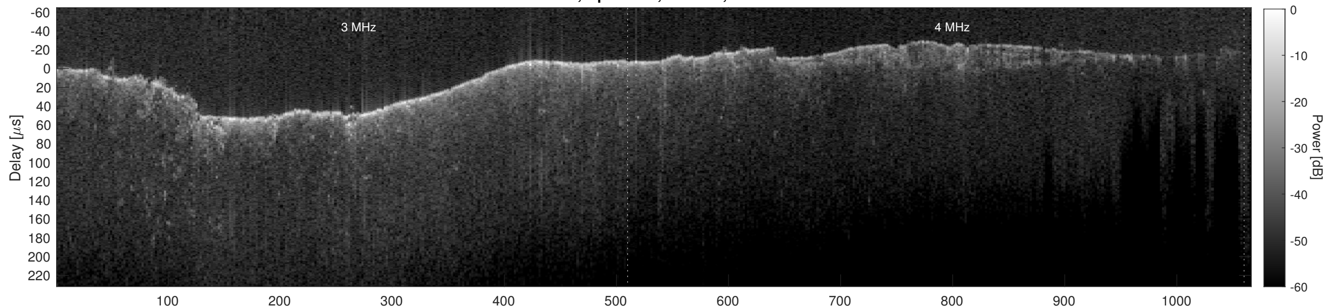
Orbit 4692, Cluttergram
