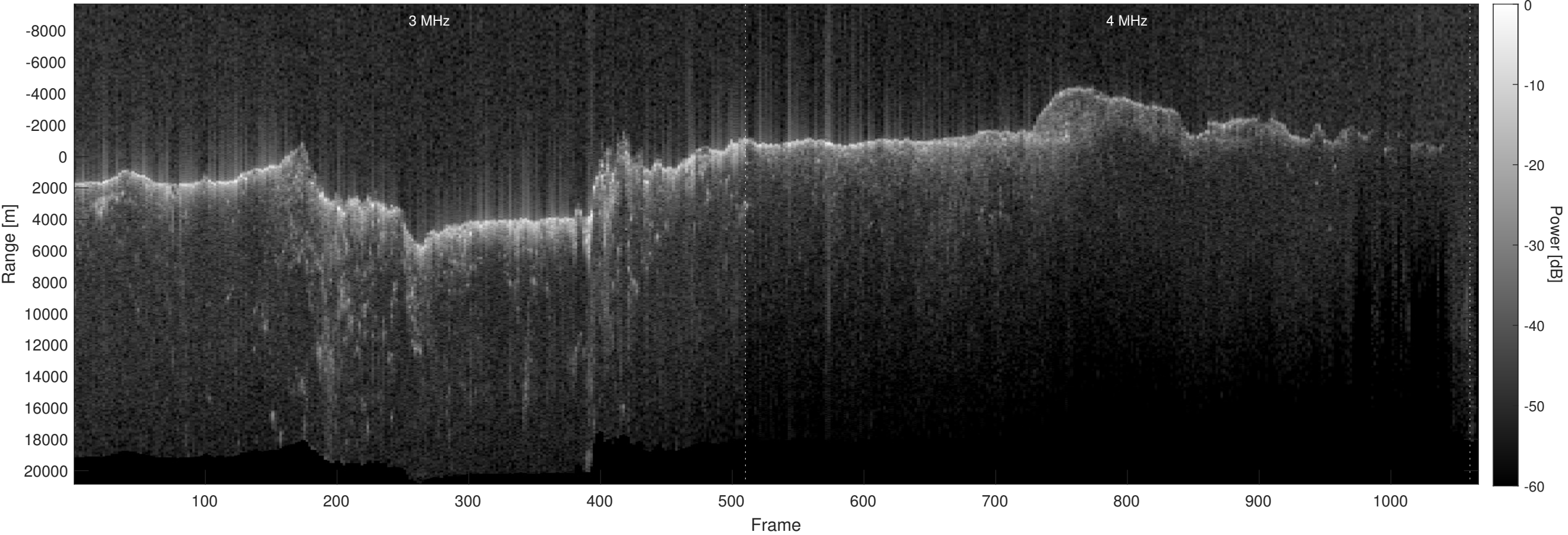
Orbit 4693, Optimized, No Window, Depth-Corrected, Channel 2
