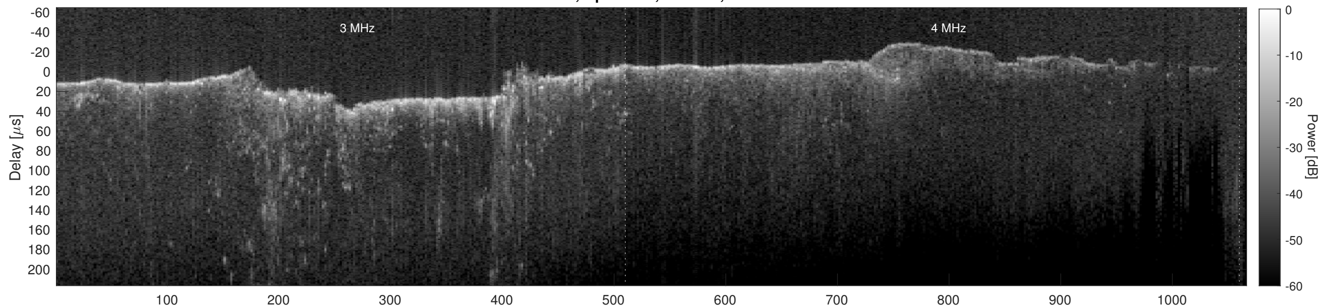
Orbit 4693, Cluttergram
